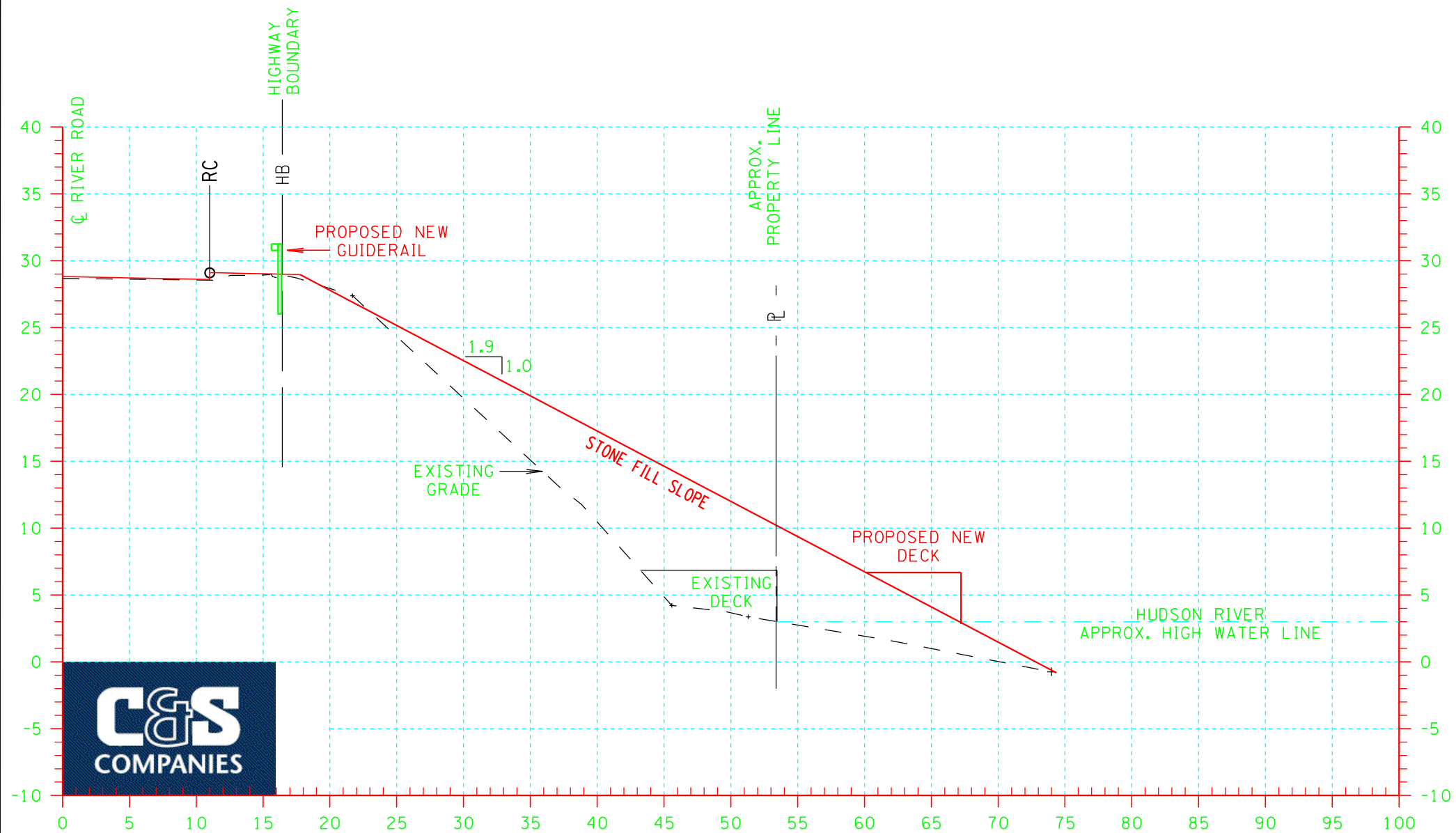
TYPICAL SLOPE SECTION
